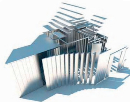
Exploded view of a Bunkerkit
